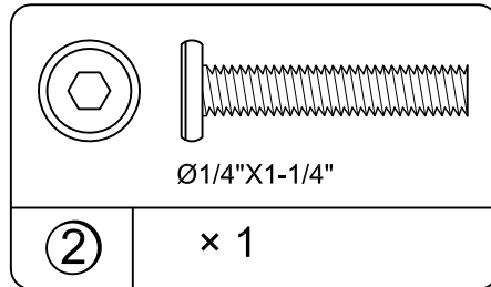
Bolt TKX1009
