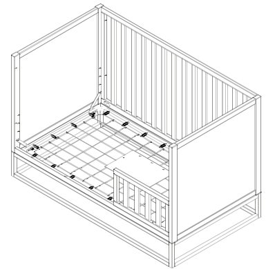
Toddler Bed
